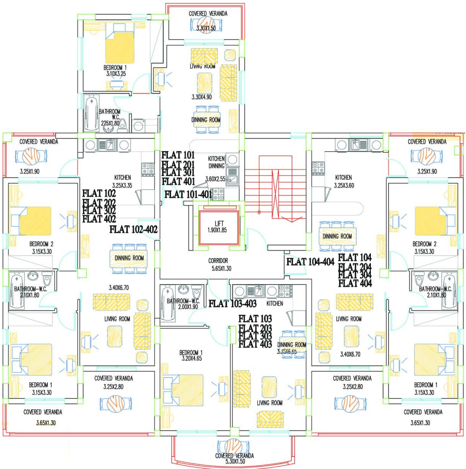
KANIKA CITY APARTMENTS BLOCK B TYPICAL FLOOR 1ST-4RTH
