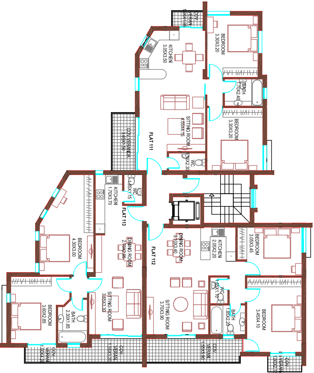
AYIOS ATHANASIOS RESIDENCE 1st FLOOR PLAN
